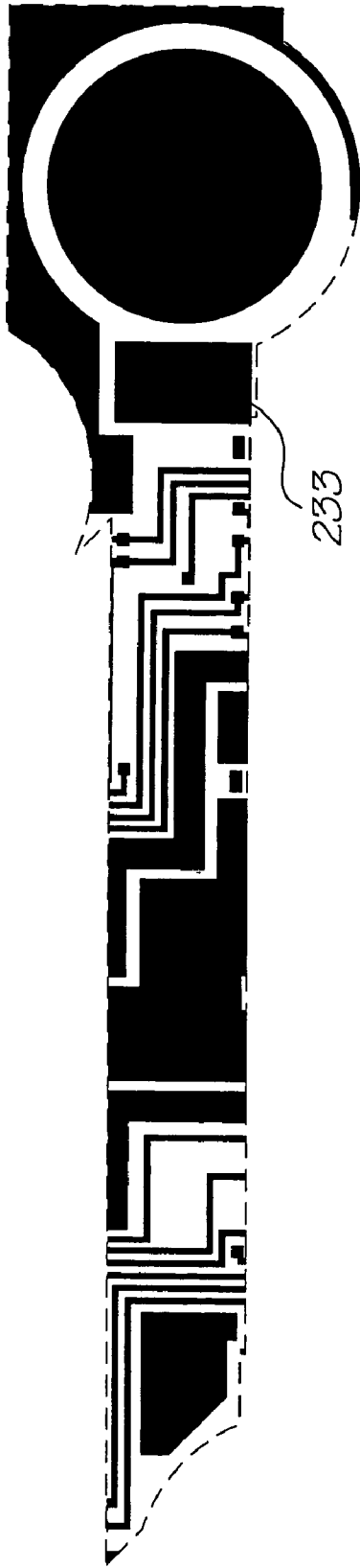
Metal 2 mask
